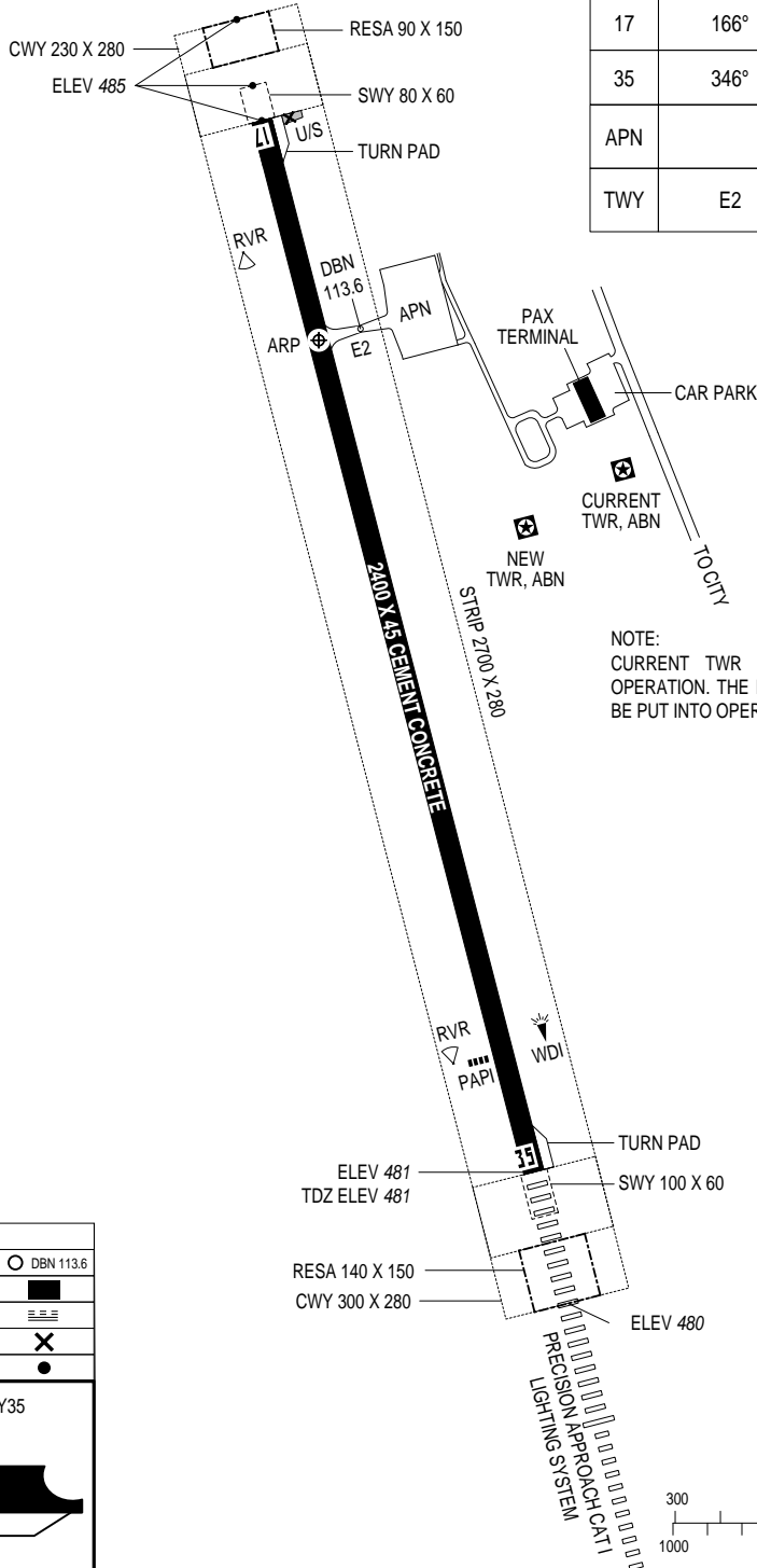
MARKING AIDS RWY 17/35 AND EXIT TWY
